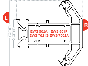
Transom T EWS 7002
