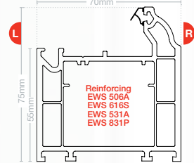
Large main frame EWS 7706
