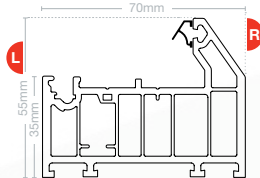
Intermediate outer frame EWS 7020 Reinforcing EWS 800P
