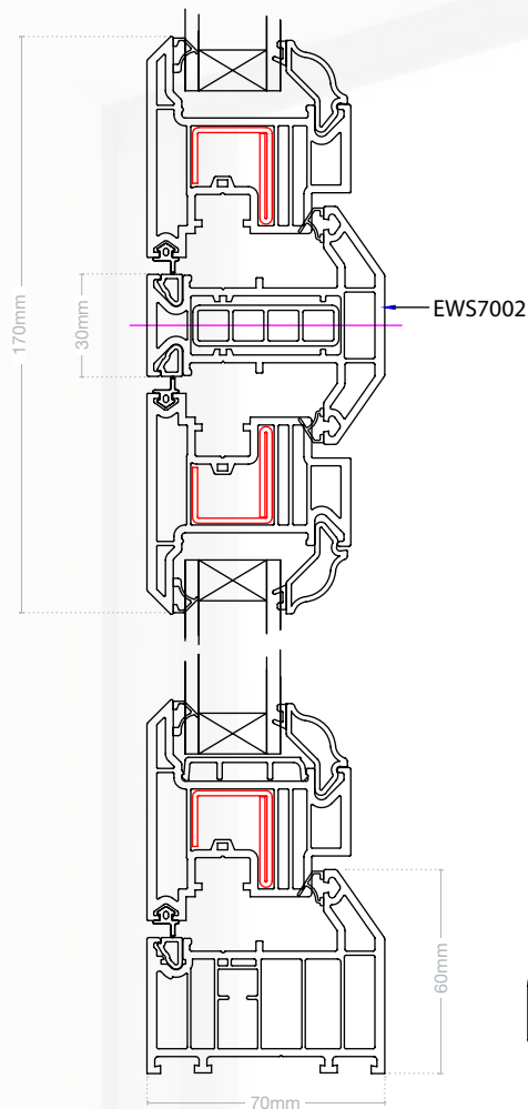
HORIZONTAL CROSS SECTION
